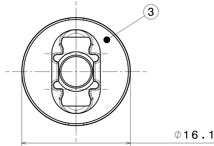
Bottom view
