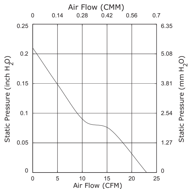
CFM-6020V-230-230
