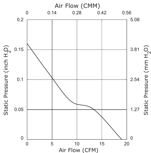
CFM-6020V-157-390
