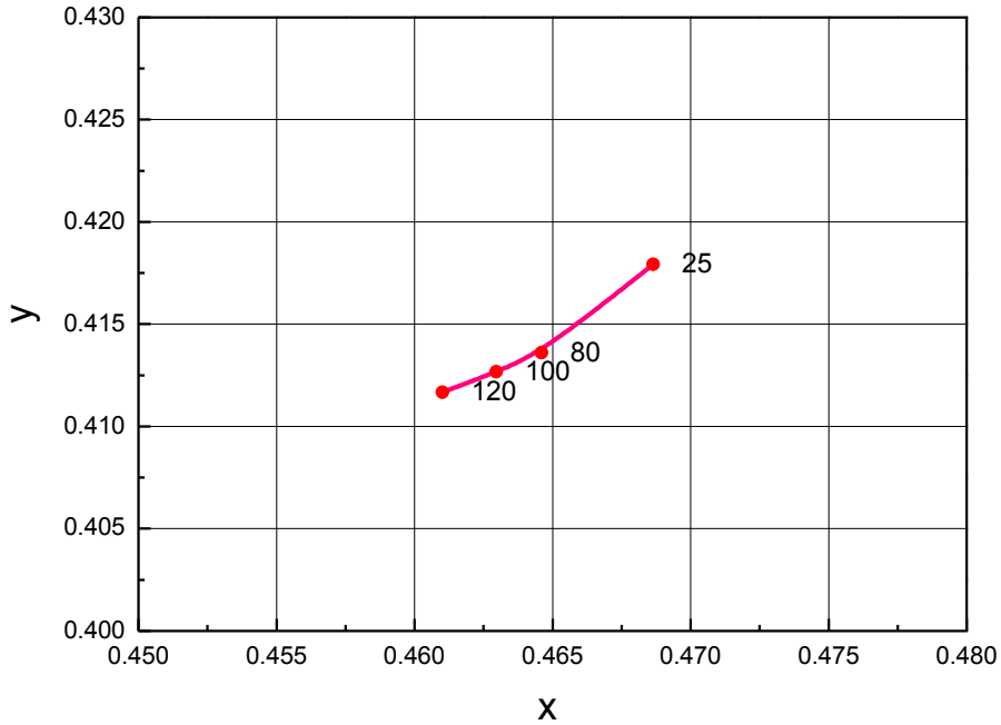
Fig 8. Chromaticity Coordinate vs. Junction Temperature, I_F=100mA (2600~3700K)
