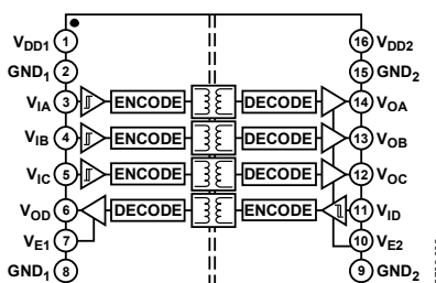
Figure 2. ADuM1401
