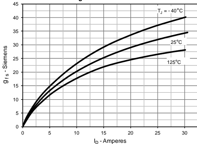
Fig. 8. Transconductance
