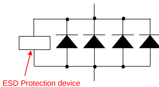
Circuit
