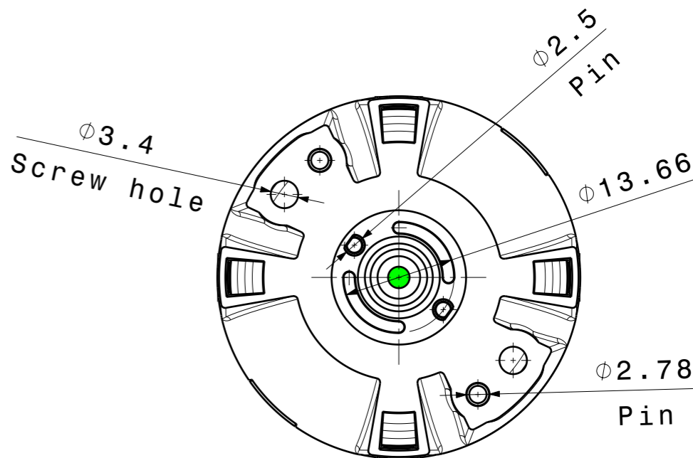
Bottom view
