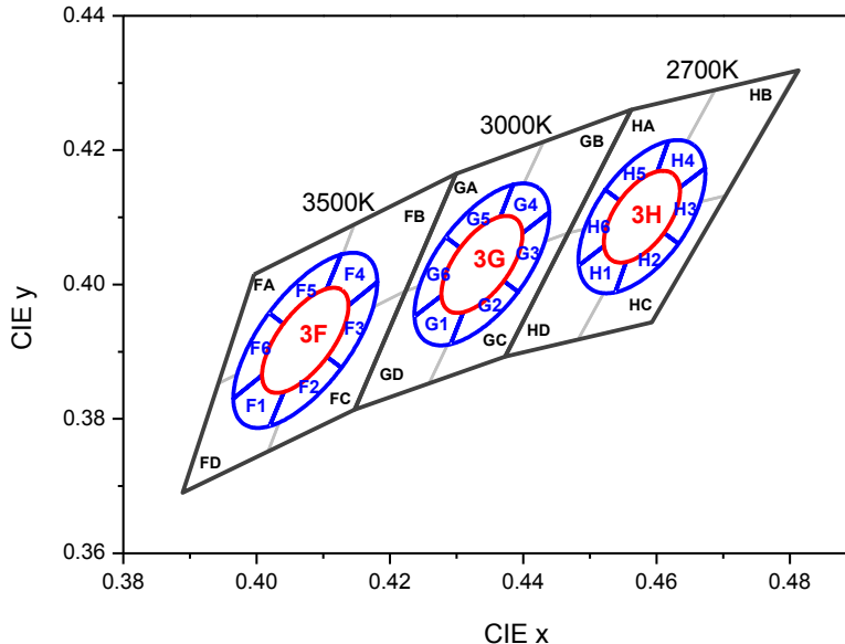
CIE Chromaticity Diagram (Warm white), T_j=25^\circ\text{C} , I_f=65\text{mA}
