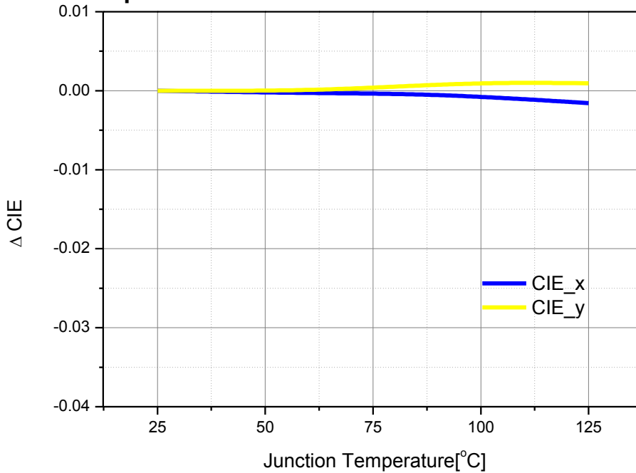
Junction Temperature vs. White ΔCIE at IF=1000mA
