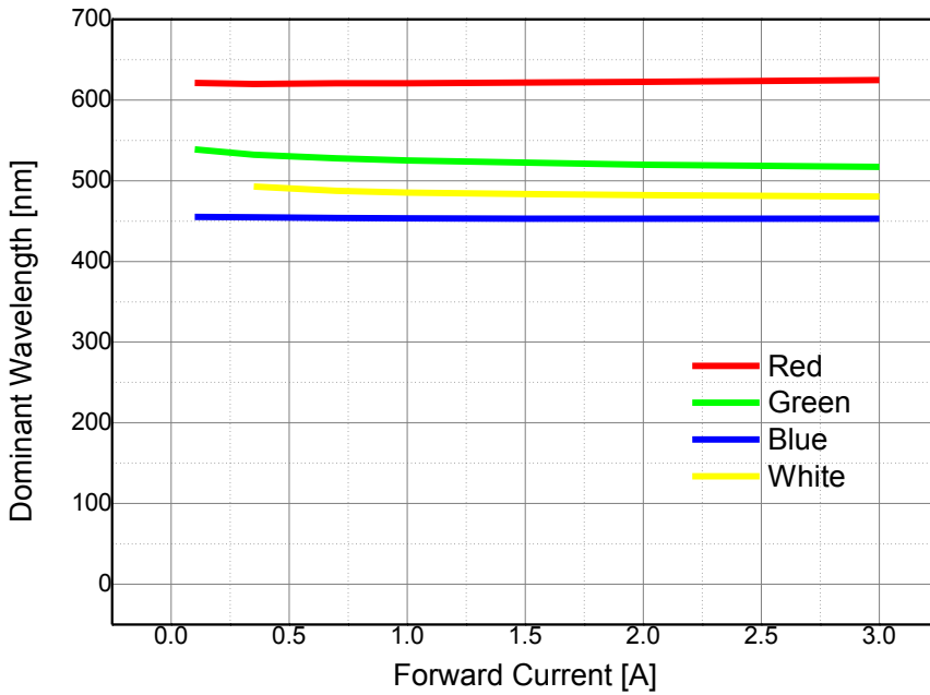
Forward Current vs Dominant Wavelength, Ta=25°C
