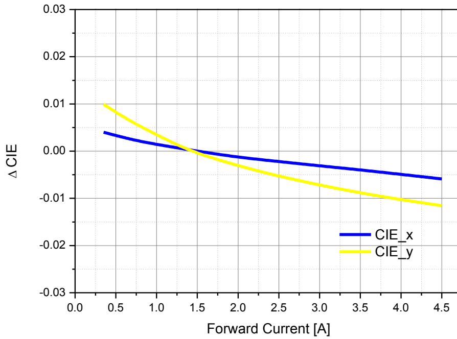
Forward Current vs \Delta CIE Ta=25°C
