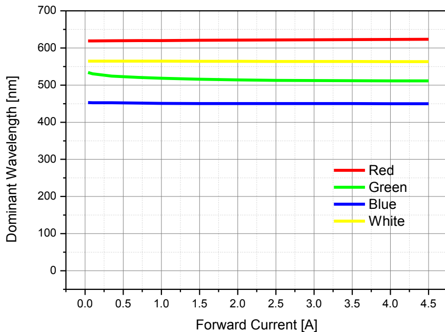
Forward Current vs Dominant Wavelength, T_a=25^\circ\text{C}
