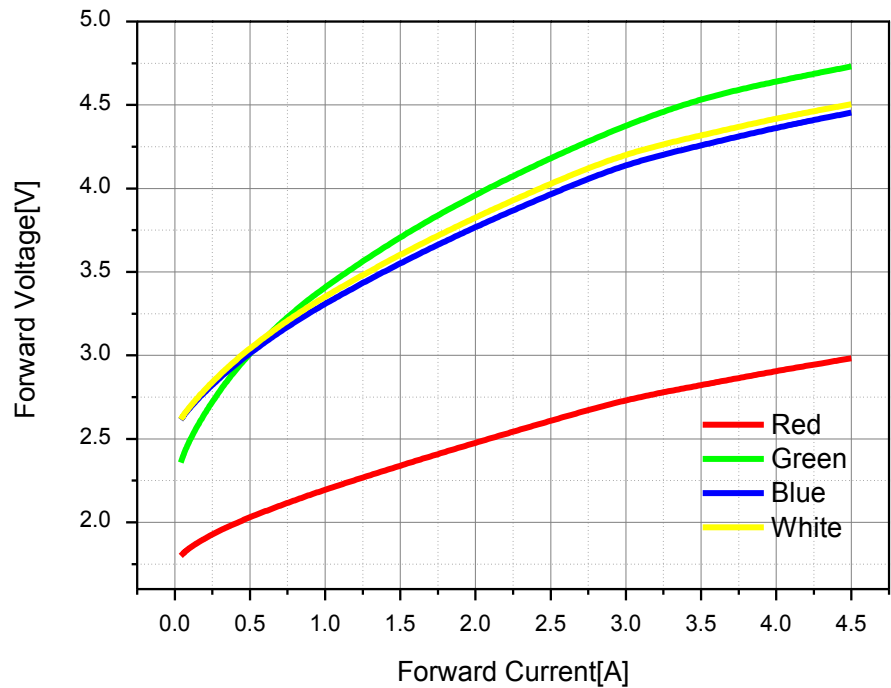
Forward Voltage vs. Forward Current, Ta=25°C
