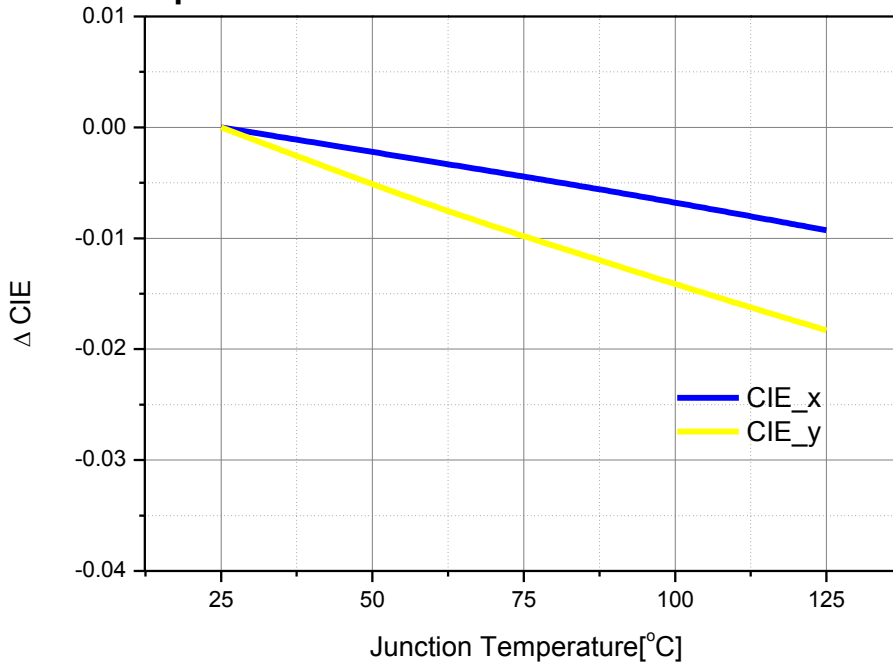
Junction Temperature vs. White \Delta CIE at IF=1400mA
