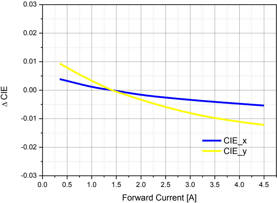
Forward Current vs ΔCIE, Ta=25°C
