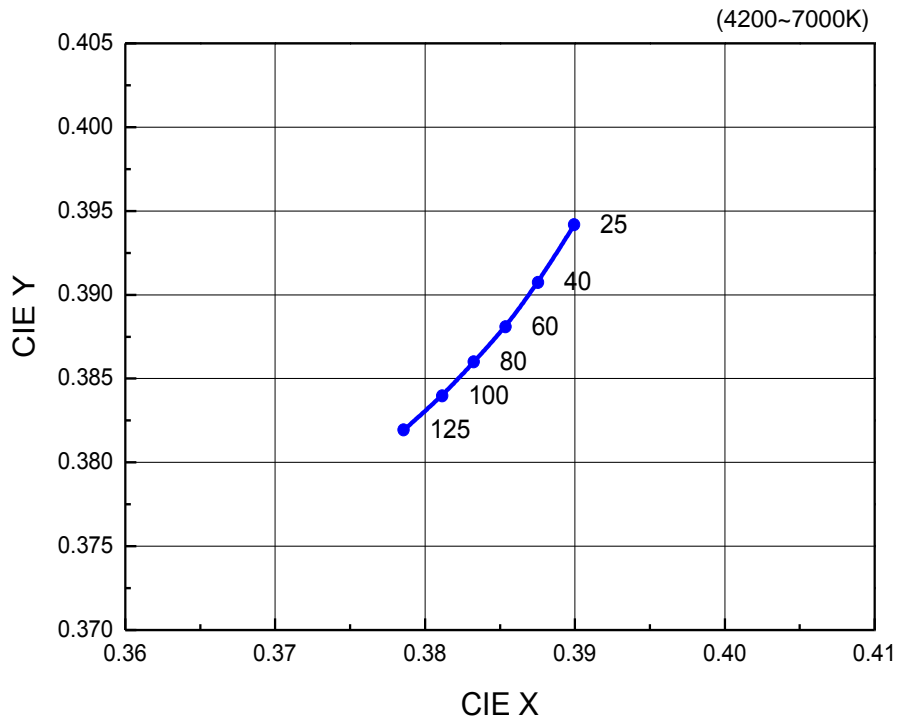
Fig 8. Chromaticity Coordinate vs. Junction Temperature, I_F=65mA
