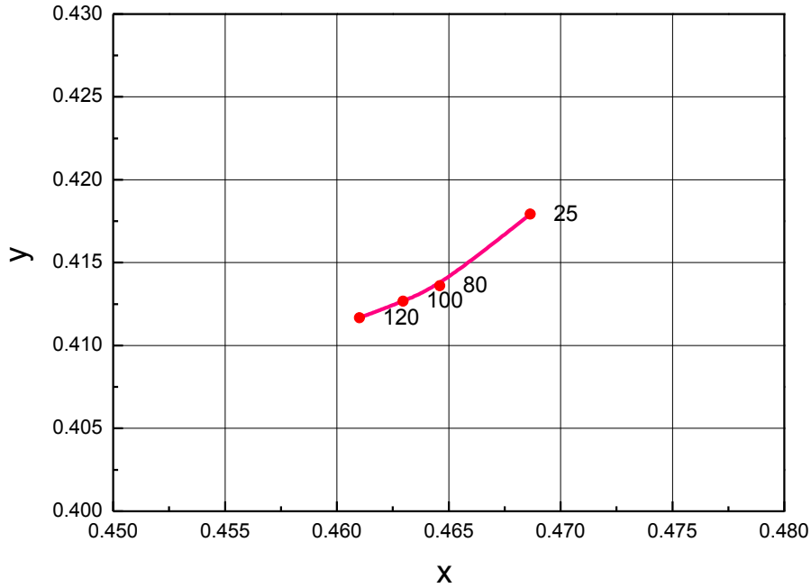
Fig 8. Chromaticity Coordinate vs. Junction Temperature, I_F=50mA
