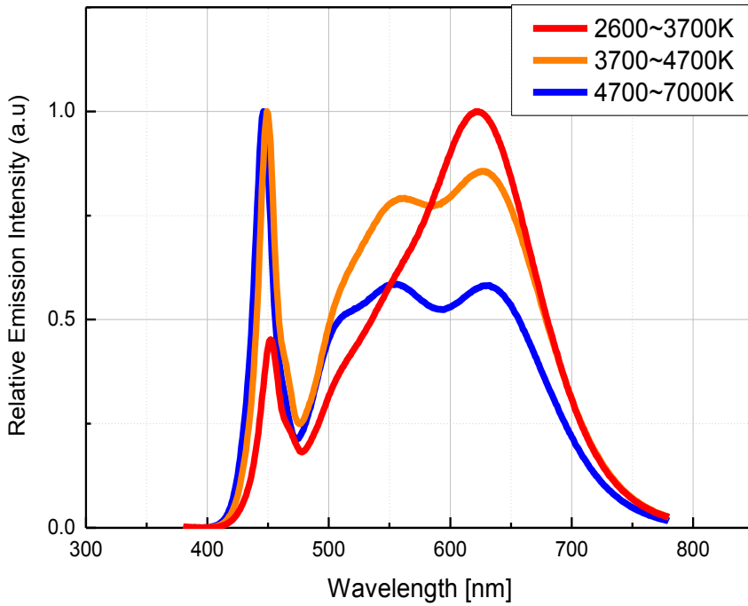
Fig 1. Color Spectrum, T_j = 25^\circ\text{C} , I_F = 50\text{mA}
