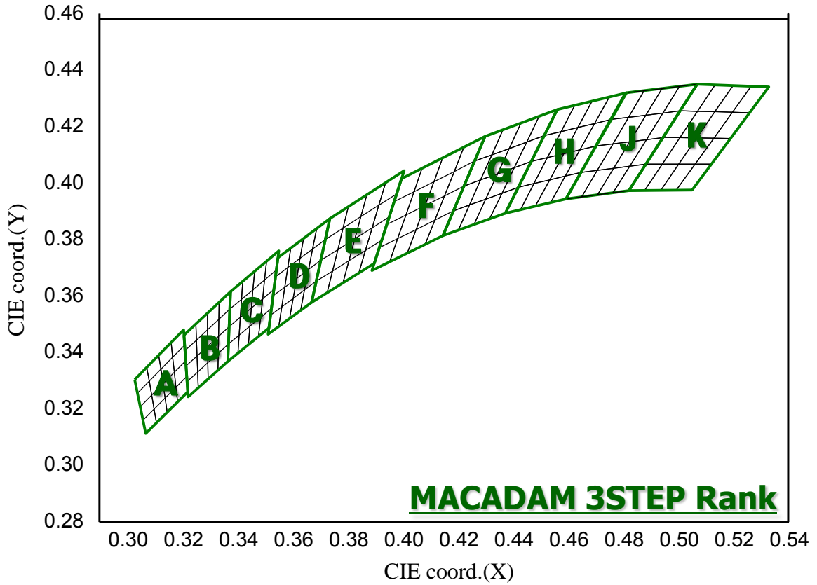
CIE Chromaticity Diagram T_j=25^\circ\text{C} , I_f=50\text{mA}
