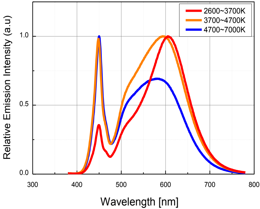
Fig 1. Color Spectrum, T_j = 25^\circ\text{C} , I_F = 50\text{mA}
