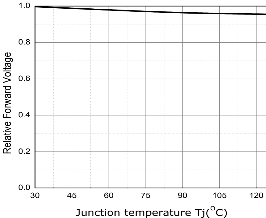
Fig 7. Junction Temperature vs. Relative Forward Voltage, I_F=50mA
