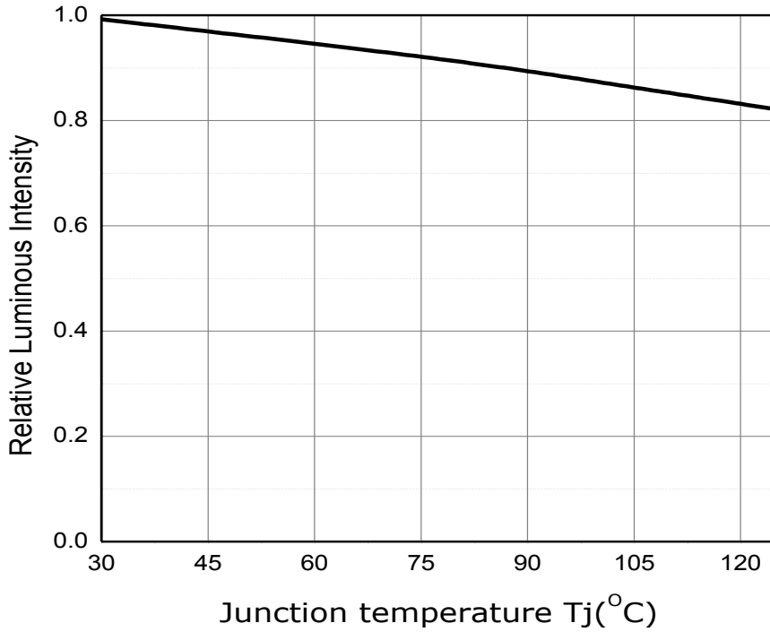
Fig 6. Junction Temperature vs. Relative Luminous Intensity, I_F=50mA
