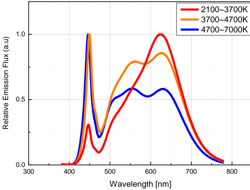
Fig 1. Color Spectrum, T_j = 25^\circ\text{C} , I_F = 50\text{mA}
