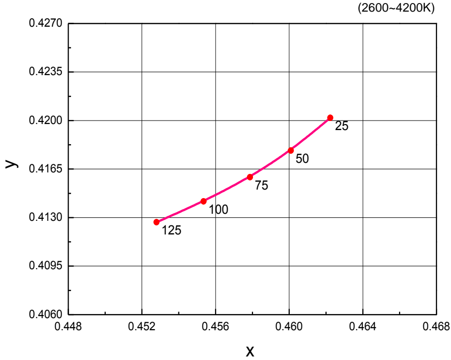
Fig 8. Chromaticity Coordinate vs. Junction Temperature, I_F=60mA
