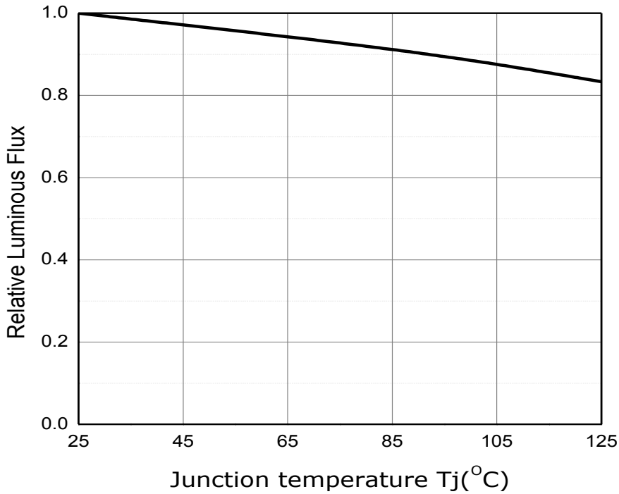
Fig 6. Junction Temperature vs. Relative Luminous Flux, I_F=60mA
