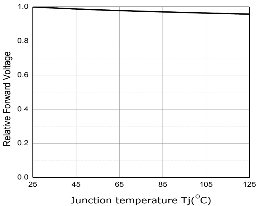
Fig 7. Junction Temperature vs. Relative Forward Voltage, I_F=60mA
