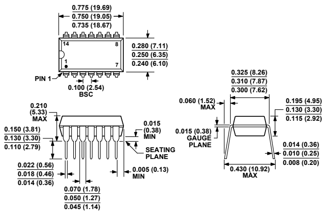
COMPLIANT TO JEDEC STANDARDS MS-001-AA CONTROLLING DIMENSIONS ARE IN INCHES; MILLIMETER DIMENSIONS (IN PARENTHESES) ARE ROUNDED-OFF INCH EQUIVALENTS FOR REFERENCE ONLY AND ARE NOT APPROPRIATE FOR USE IN DESIGN. CORNER LEADS MAY BE CONFIGURED AS WHOLE OR HALF LEADS.
