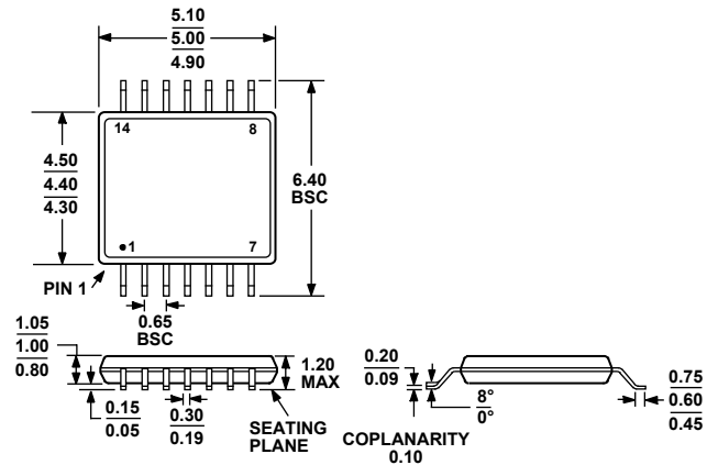
COMPLIANT TO JEDEC STANDARDS MO-153-AB-1
