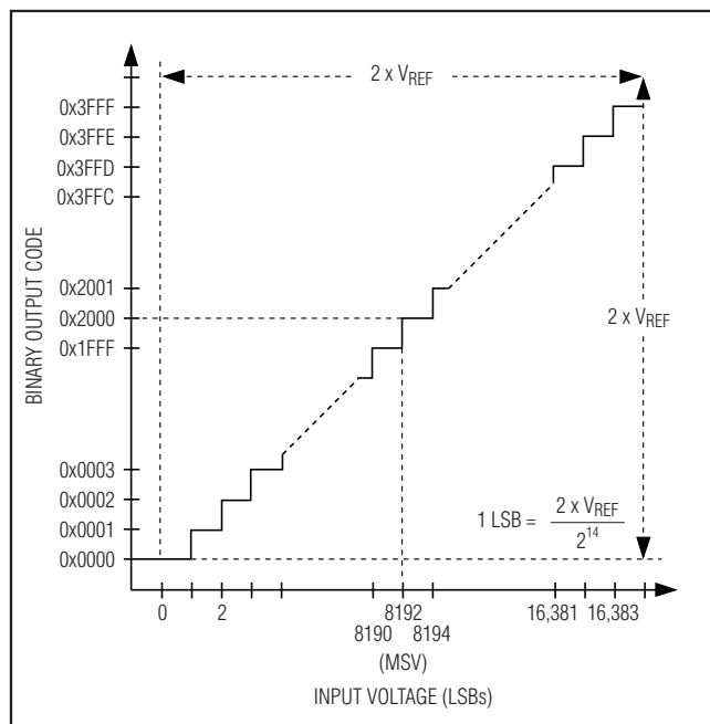
Figure 11. 0 to +5\text{V} Unipolar Transfer Function
