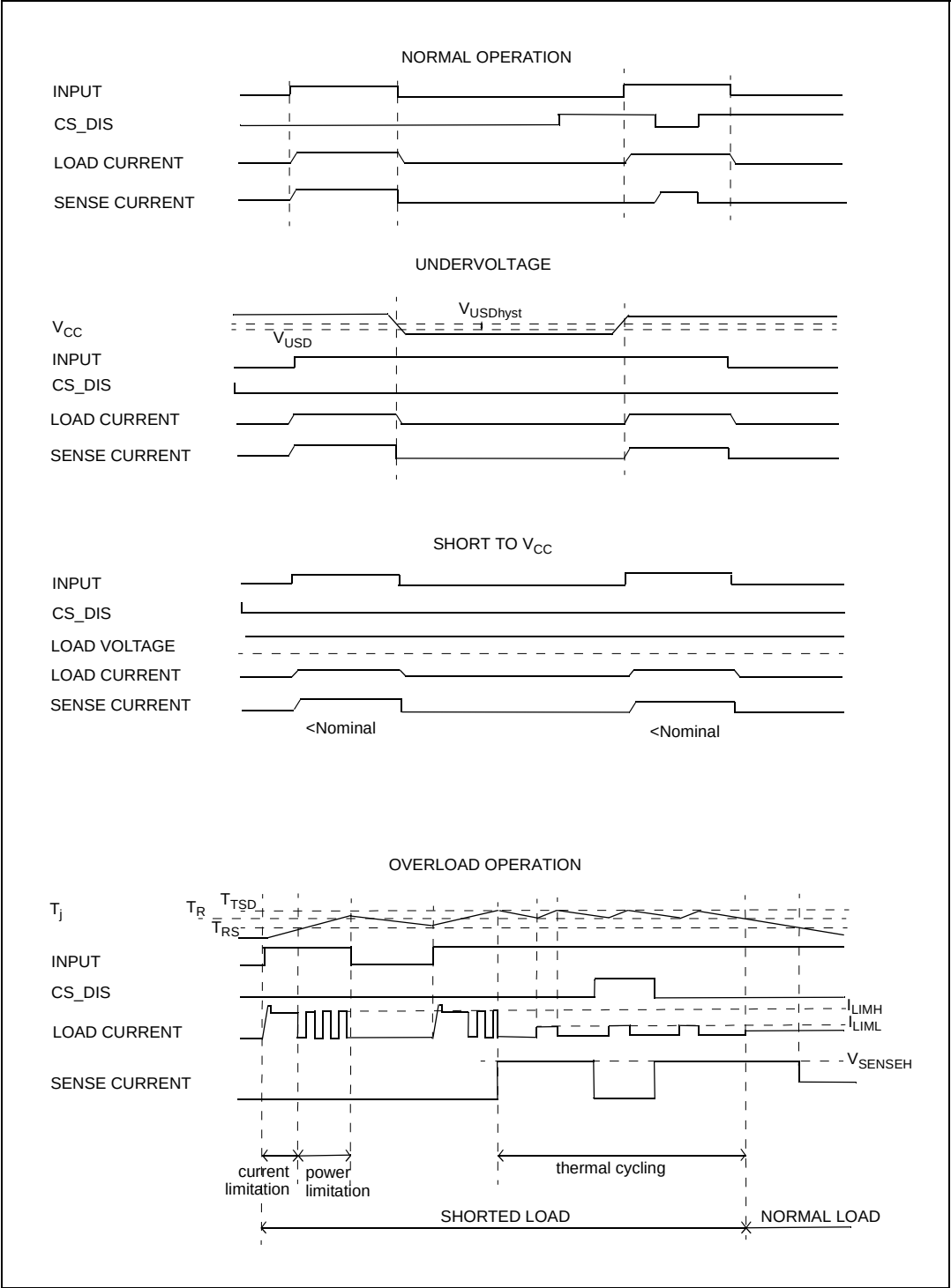
Figure 26. Waveforms
