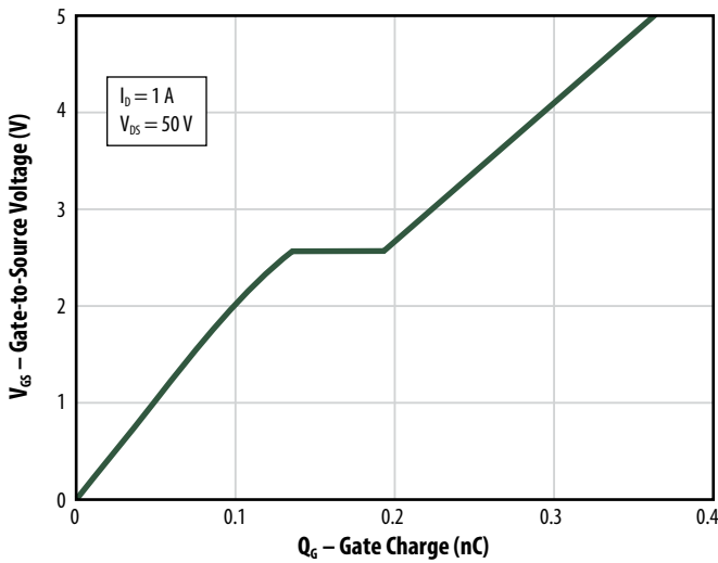
Figure 6: Gate Charge
