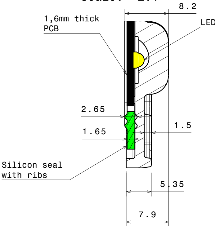
Section view B-B Scale: 2:1
