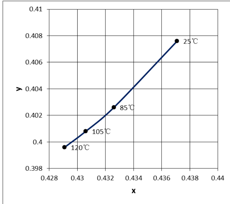
Fig 8. Chromaticity Coordinate vs. Junction Temperature, I_F=65mA (2700~3500K)
