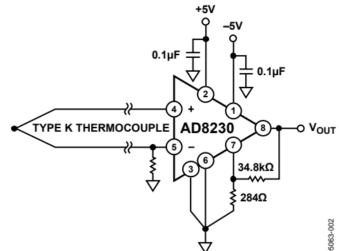
Figure 3. Thermocouple Measurement
