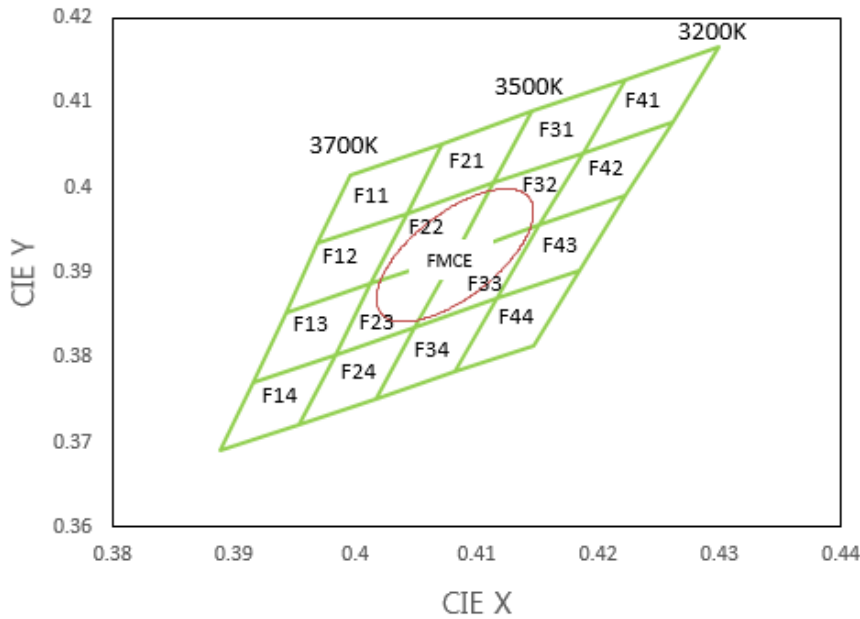
CIE Chromaticity Diagram (Warm white), T_j=25^\circ\text{C} , I_f=150\text{mA}
