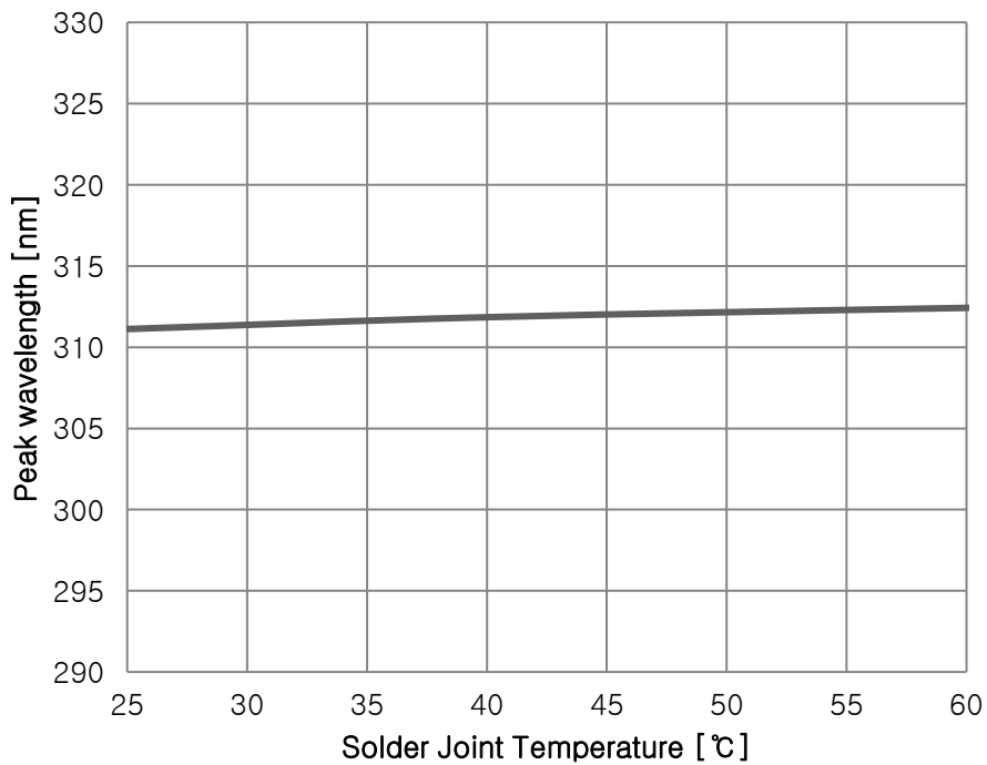
Fig 6. Surface Temperature vs. Peak Wavelength, I_F=20\text{mA}
