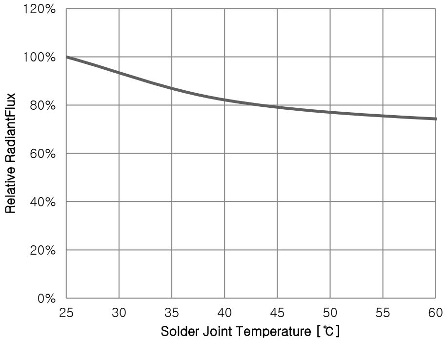
Fig 5. Surface Temperature vs. Relative Radiant Flux, I_F=20\text{mA}
