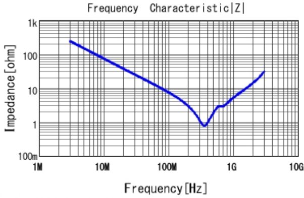
■ GR442QR73D221KW01 |Z| DC0V, 25degC
