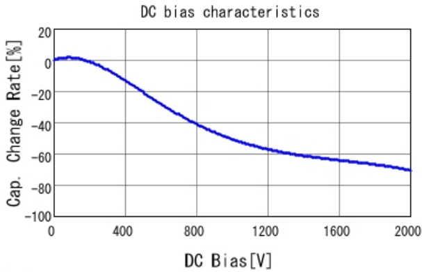
■ GR442QR73D221KW01 C-DC bias capchange, 25.0degC, AC1V
