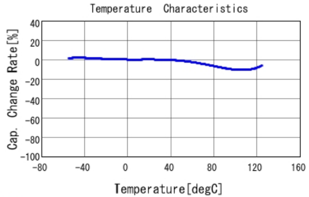
■ GR442QR73D221KW01 C-Temp. capchange, DC0V, AC1Vrms
