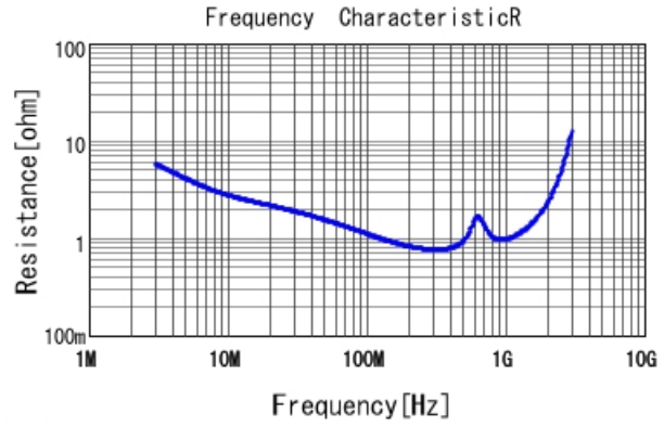
■ GR442QR73D221KW01 R DC0V, 25degC
