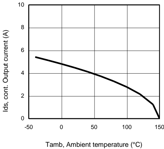
Figure 7 – Max. output current (A) Vs Ambient temperature (°C) R_{th}=50^{\circ}C/W
