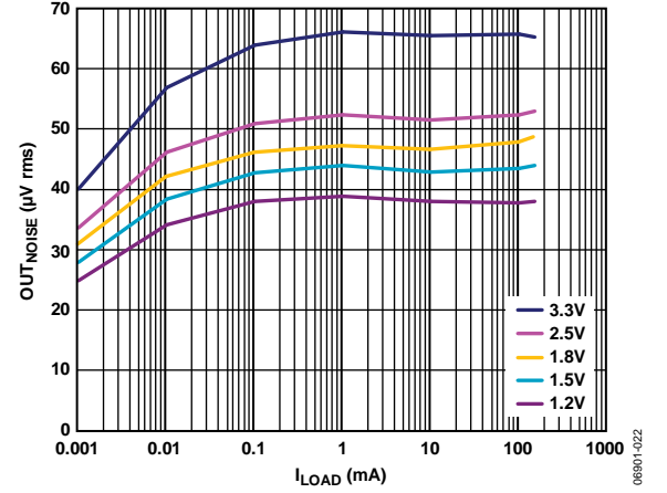
Figure 22. Output Noise vs. Load Current and Output Voltage, V_{IN} = 5V , C_{OUT} = 1\ \mu\text{F}
