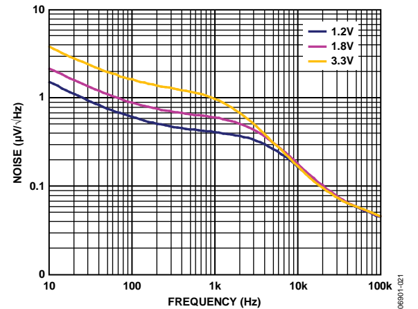
Figure 21. Output Noise Spectrum, V_{IN} = 5V , I_{LOAD} = 10\text{ mA} , C_{OUT} = 1\ \mu\text{F}
