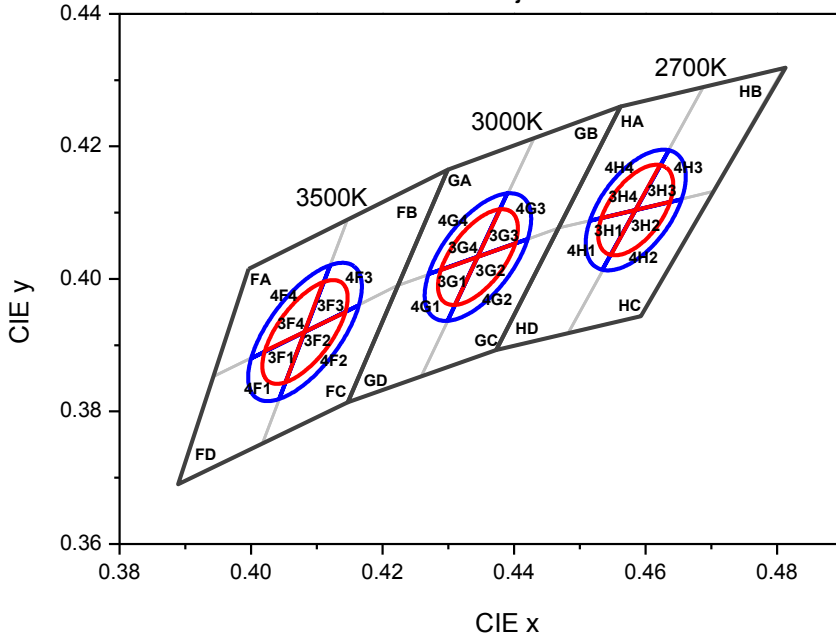
CIE Chromaticity Diagram (Warm white), T_j=25^\circ\text{C} , I_f=65\text{mA}
