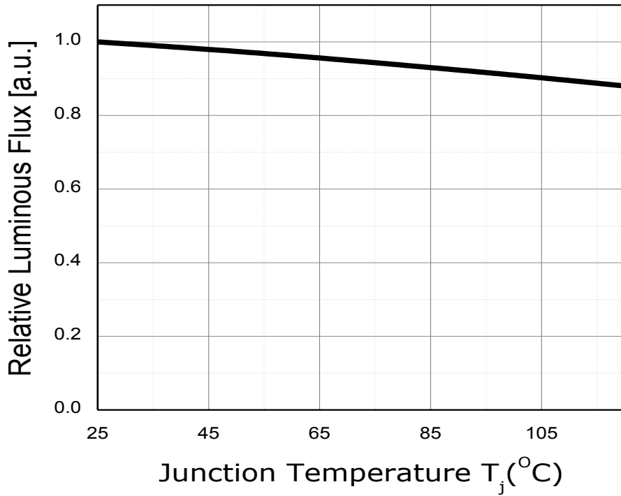
Fig 6. Junction Temperature vs. Relative Luminous Flux, I_F=65mA
