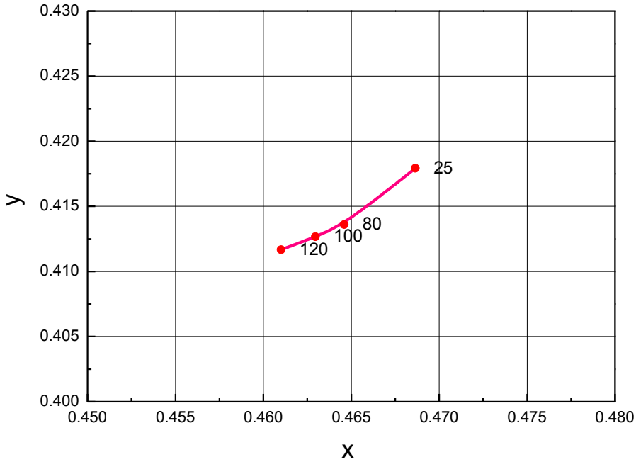
Fig 8. Chromaticity Coordinate vs. Junction Temperature, I_F=50\text{mA}
