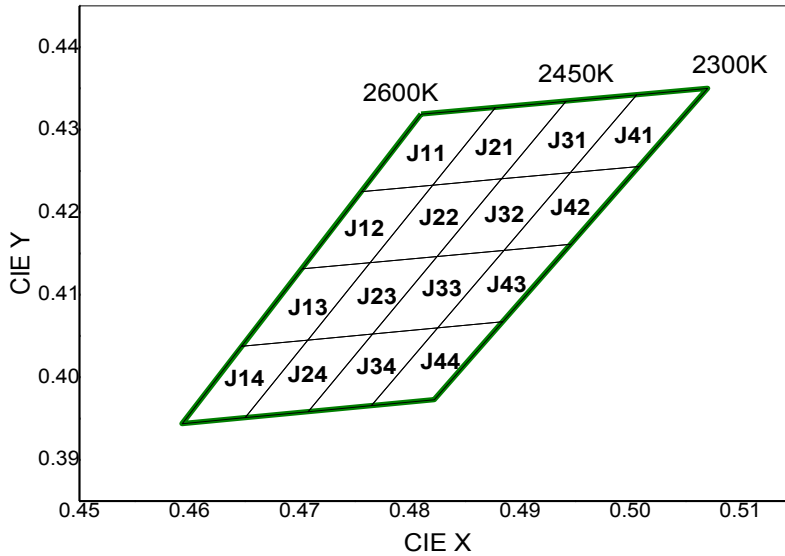
CIE Chromaticity Diagram (Warm white), T_j=25^\circ\text{C} , I_f=50\text{mA}
