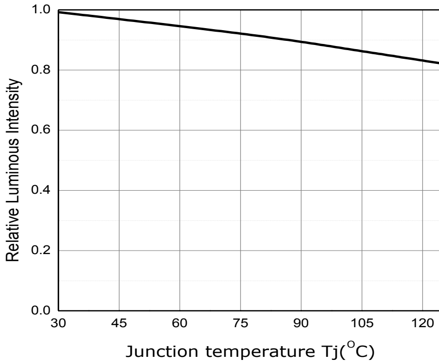
Fig 6. Junction Temperature vs. Relative Luminous Intensity, I_F=50\text{mA}
