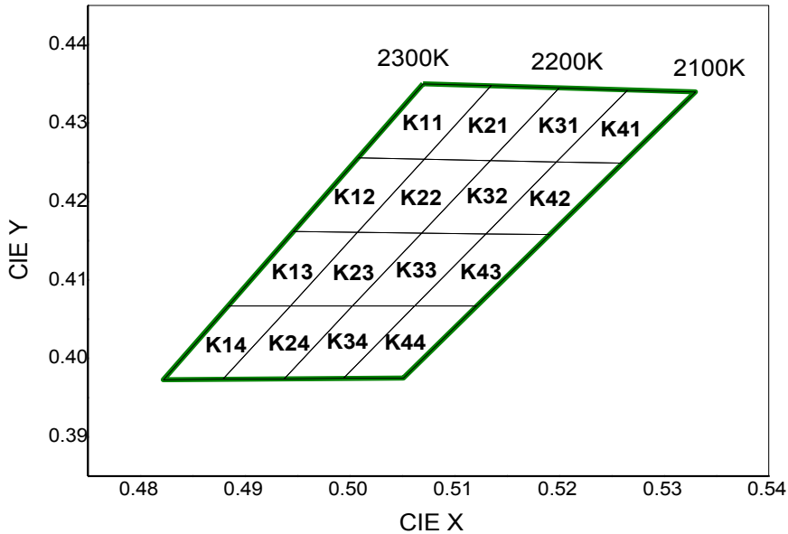
CIE Chromaticity Diagram (Warm white), T_j=25^\circ\text{C} , I_f=50\text{mA}
