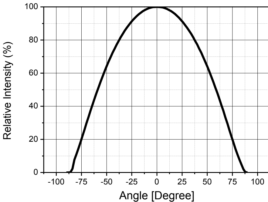
Fig 2. Radiant Pattern, T_j = 25^\circ\text{C} , I_F = 50\text{mA}
