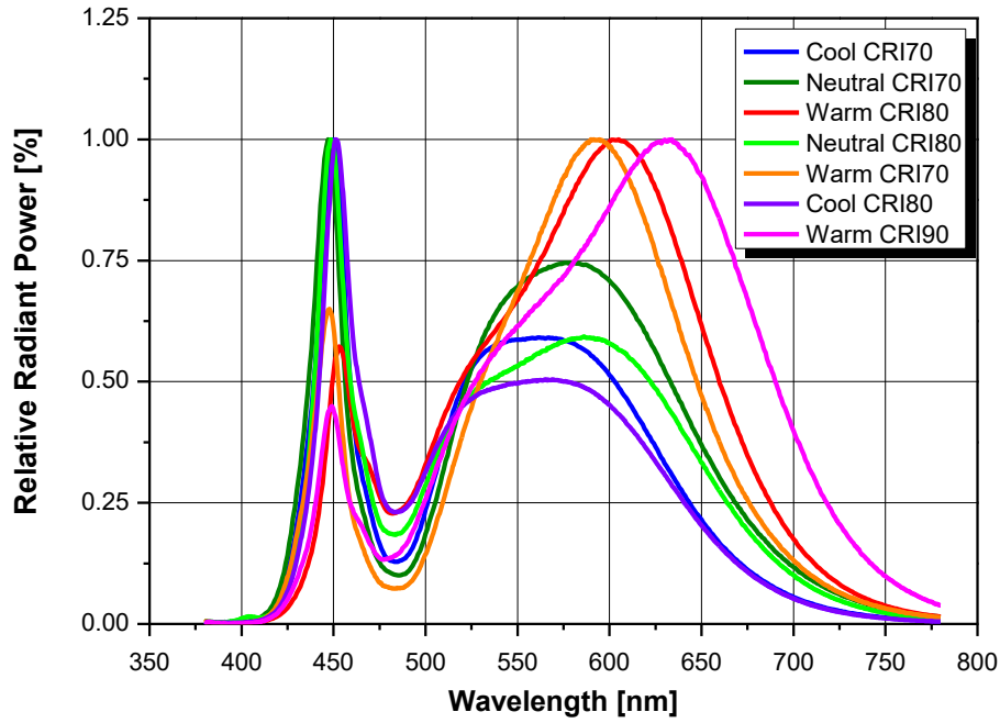
Fig 1. Color Spectrum
