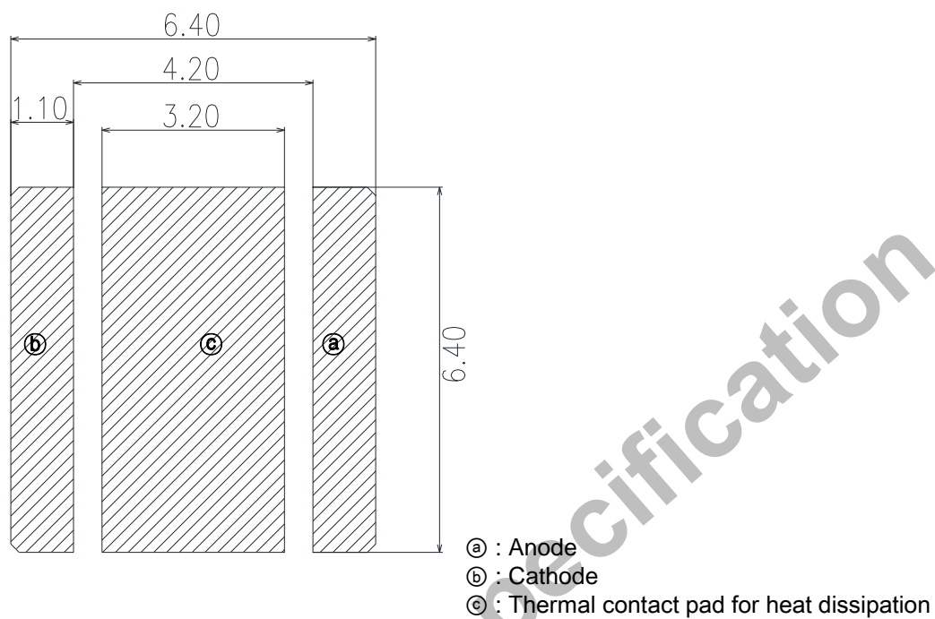
Recommended PCB solder pad
