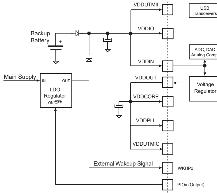
Figure 23-4. Battery Backup
