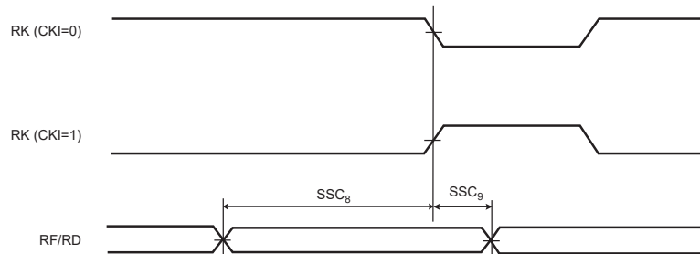
Figure 59-35. SSC Receiver RK and RF in Input
