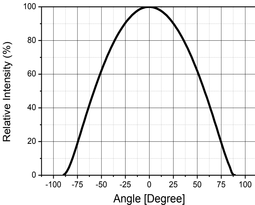
Fig 2. Radiant Pattern, T_j = 25^\circ\text{C} , I_F = 65\text{mA}
