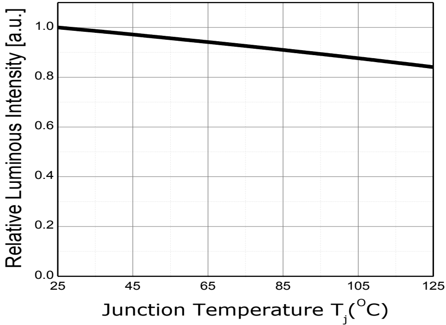
Fig 6. Junction Temperature vs. Relative Luminous Intensity, I_F=20mA
