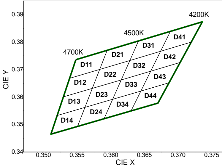
CIE Chromaticity Diagram (Neutral white), T_j=25^\circ\text{C} , I_f=20\text{mA}
