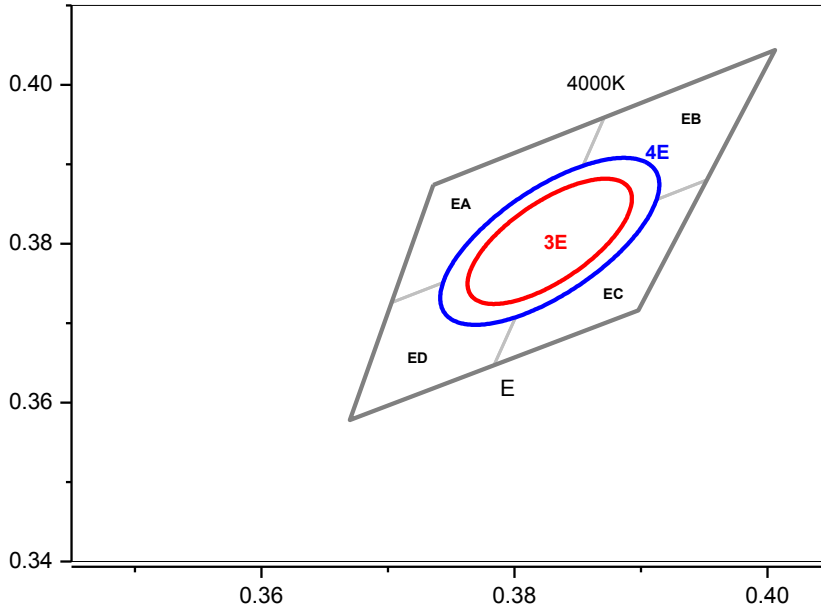
CIE Chromaticity Diagram T_j=25^\circ\text{C} , I_F=150\text{mA}
