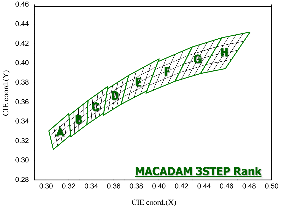
CIE Chromaticity Diagram T_j=25^\circ\text{C} , I_f=65\text{mA}
