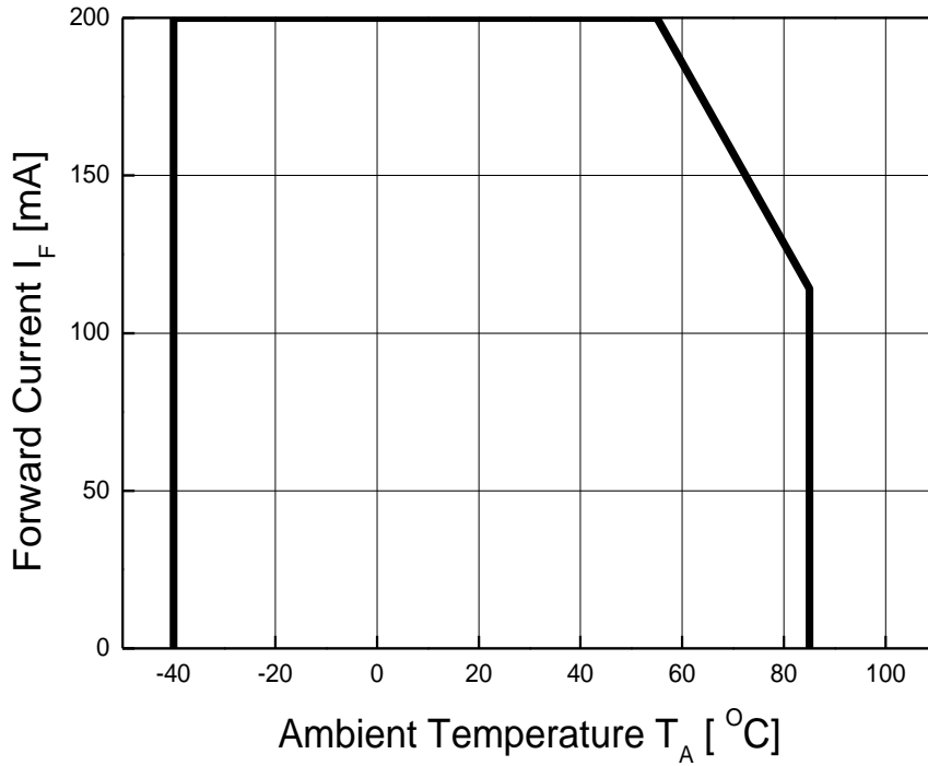
Fig 9. Ambient Temperature vs. Maximum Forward Current, T_{j\_max} = 125\text{ }^{\circ}\text{C}
