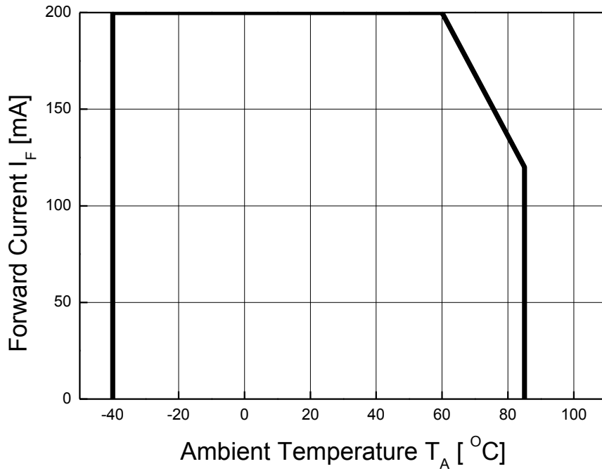
Fig 9. Ambient Temperature vs. Maximum Forward Current, T_{j\_max} = 125\text{ }^{\circ}\text{C}
