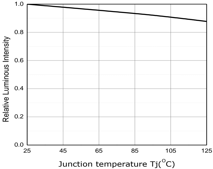
Fig 6. Junction Temperature vs. Relative Luminous Intensity, I_F=65mA
