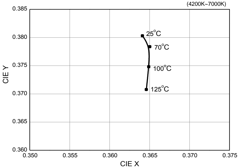
Fig 8. Chromaticity Coordinate vs. Junction Temperature, I_F=65mA
