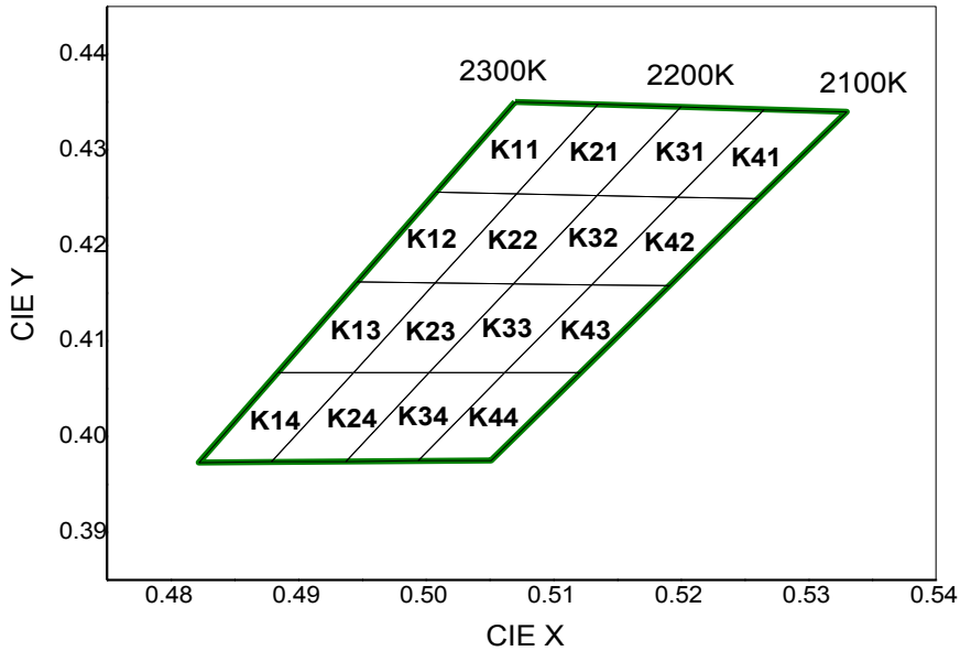
CIE Chromaticity Diagram (Warm white), T_j=25^\circ\text{C} , I_f=65\text{mA}
