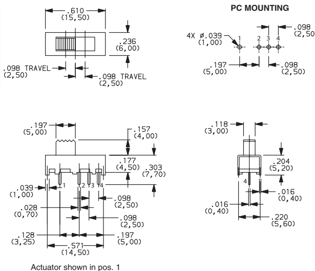
OS103012MU2QP1 SP3T
