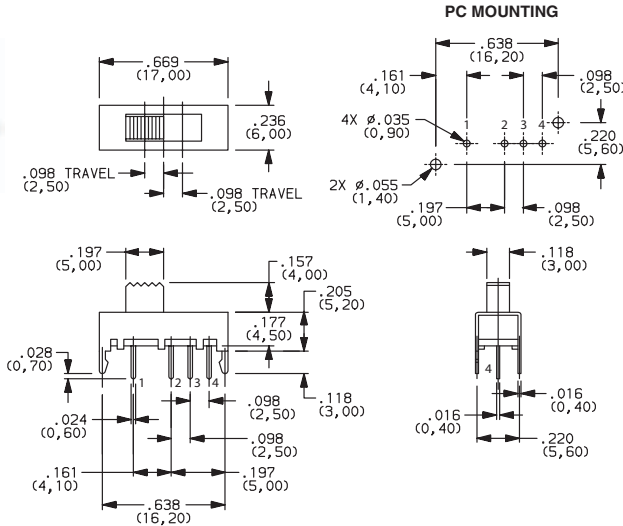
OS103012MU1QP1 SP3T
