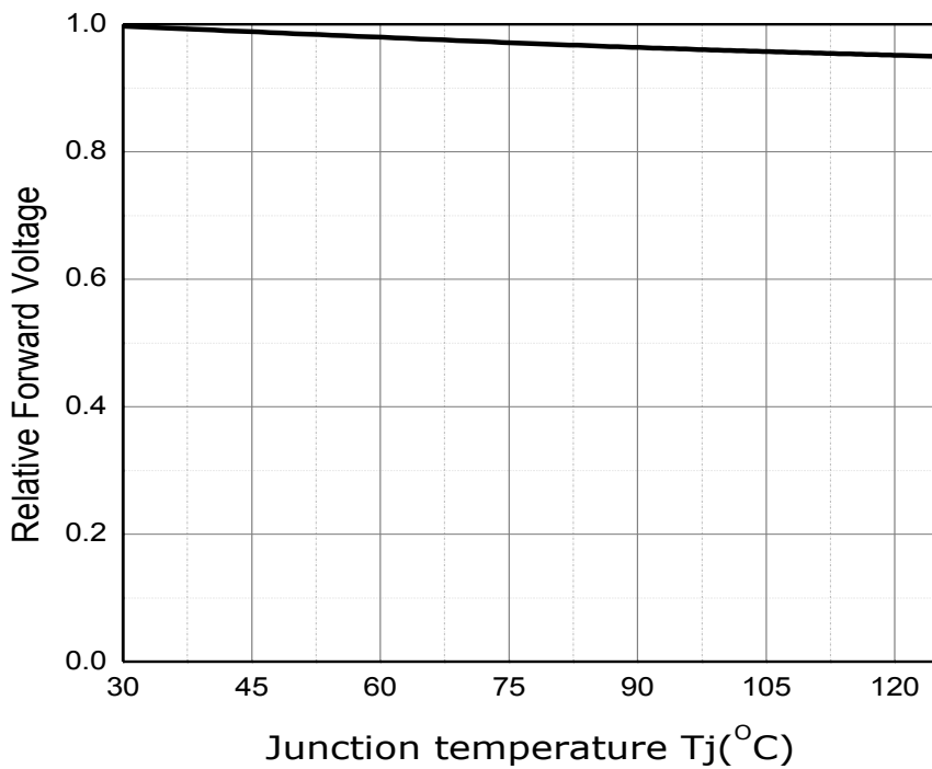
Fig 7. Junction Temperature vs. Relative Forward Voltage, I_F=100mA
