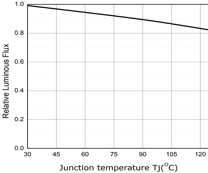
Fig 6. Junction Temperature vs. Relative Luminous Flux, I_F=100mA
