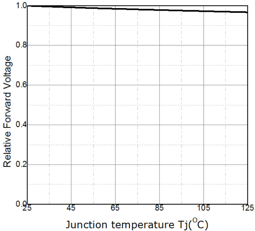
Fig 7. Junction Temperature vs. Relative Forward Voltage, I_F=120mA
