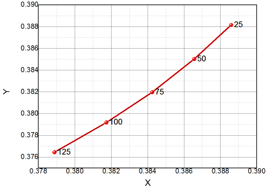
Fig 8. Chromaticity Coordinate vs. Junction Temperature, I_F=120mA (2600~4200K)
