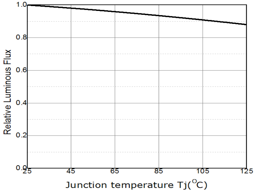
Fig 6. Junction Temperature vs. Relative Luminous Flux, I_F=120mA
