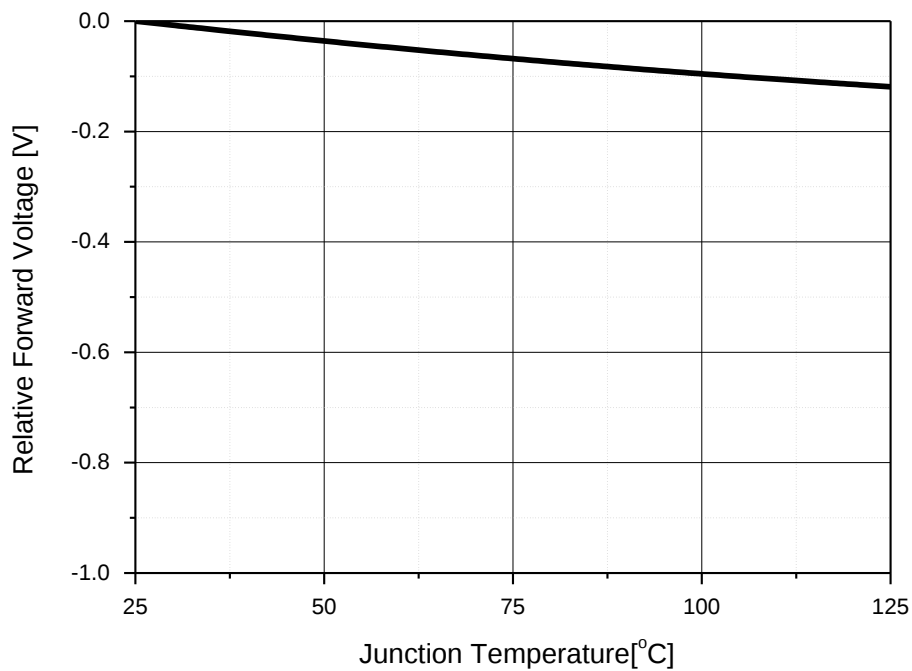
Junction Temperature vs. Relative Forward Voltage at I_F=350\text{mA}
