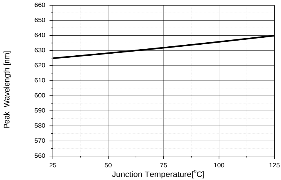
Junction Temperature vs. Peak Wavelength at IF=350mA
