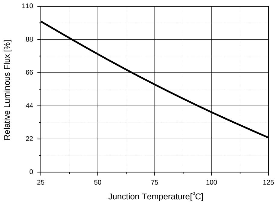
Junction Temperature vs. Relative Light Output at I_F=350\text{mA}
