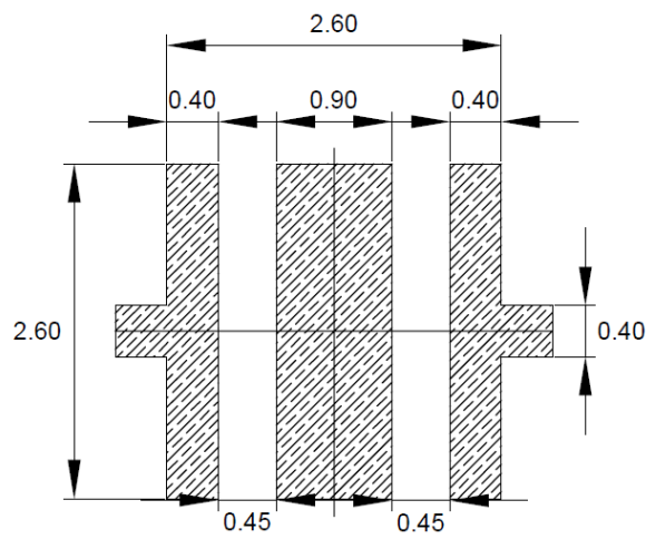
Recommended Stencil Pattern
