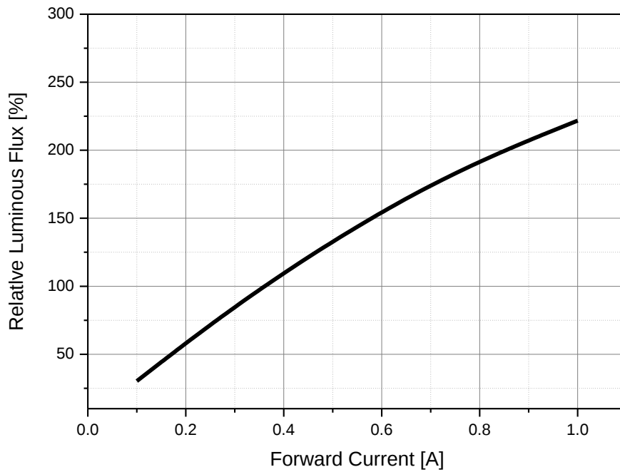
Forward Current vs. Normalized Relative Luminous Flux, T_a=25^{\circ}\text{C}
