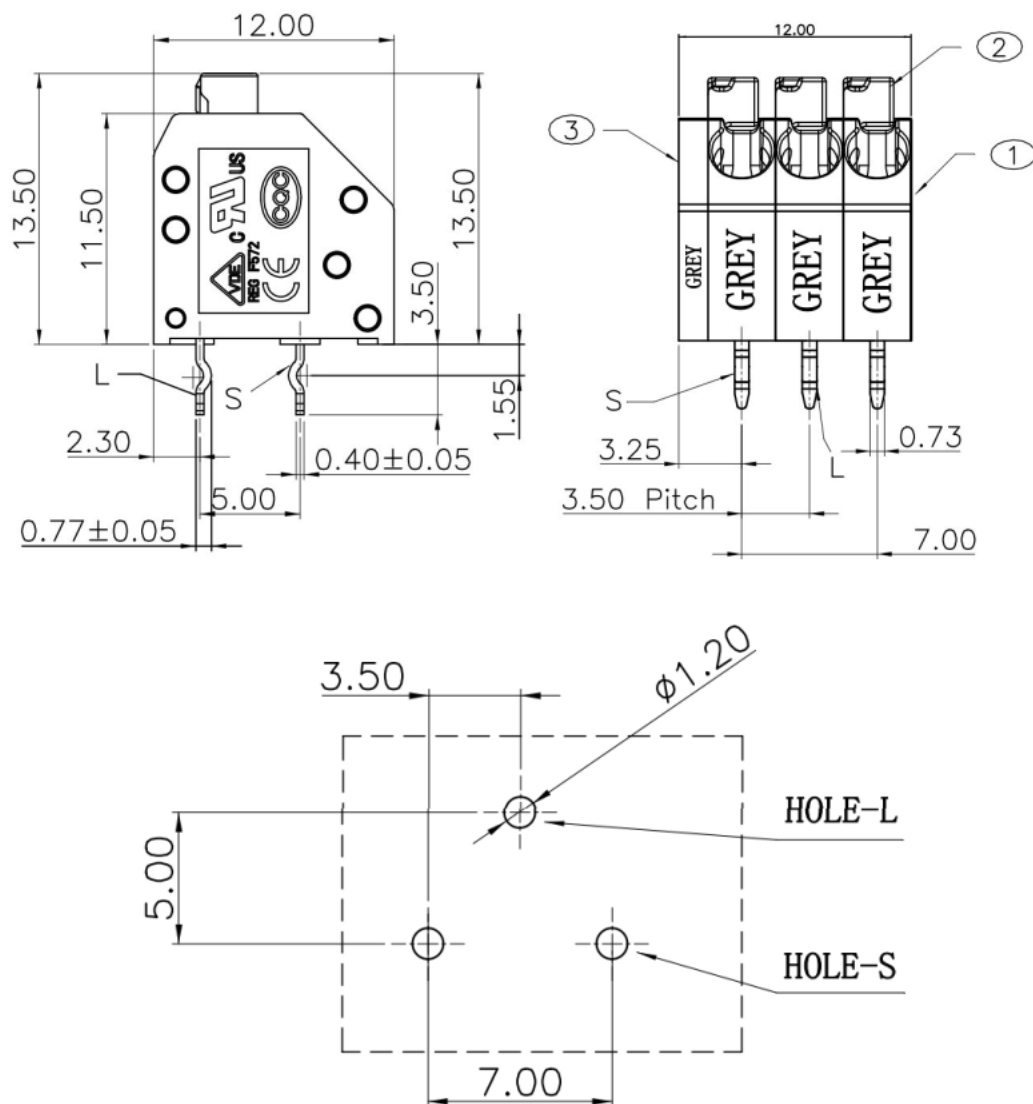
RECOMMENDED PCB LAYOUT(TOP VIEW) TOLERANCE:±0.05
