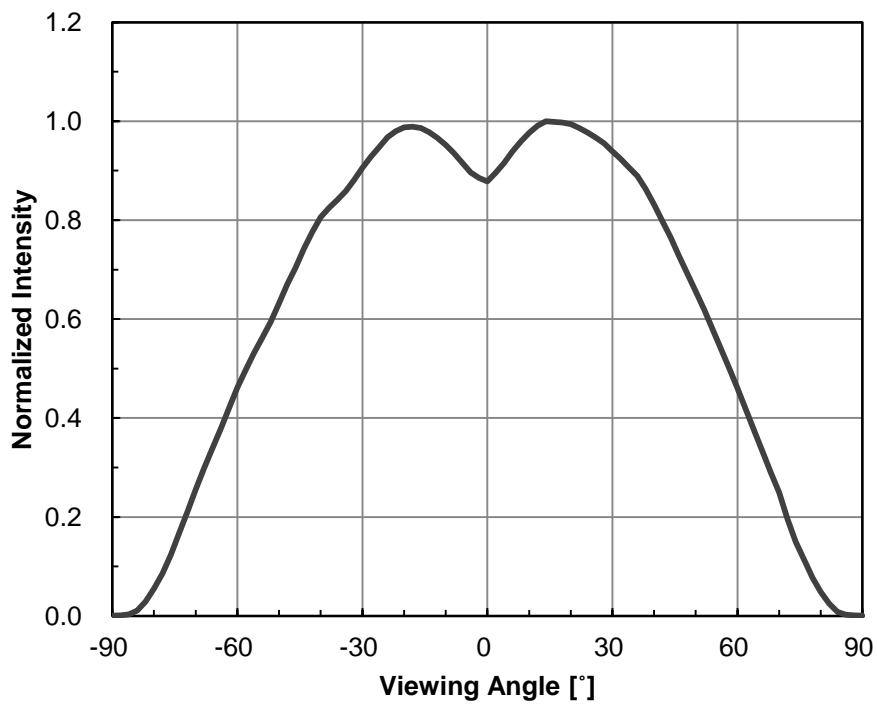
Fig 8. Typical Spatial Distribution, I_F=600\text{mA}
